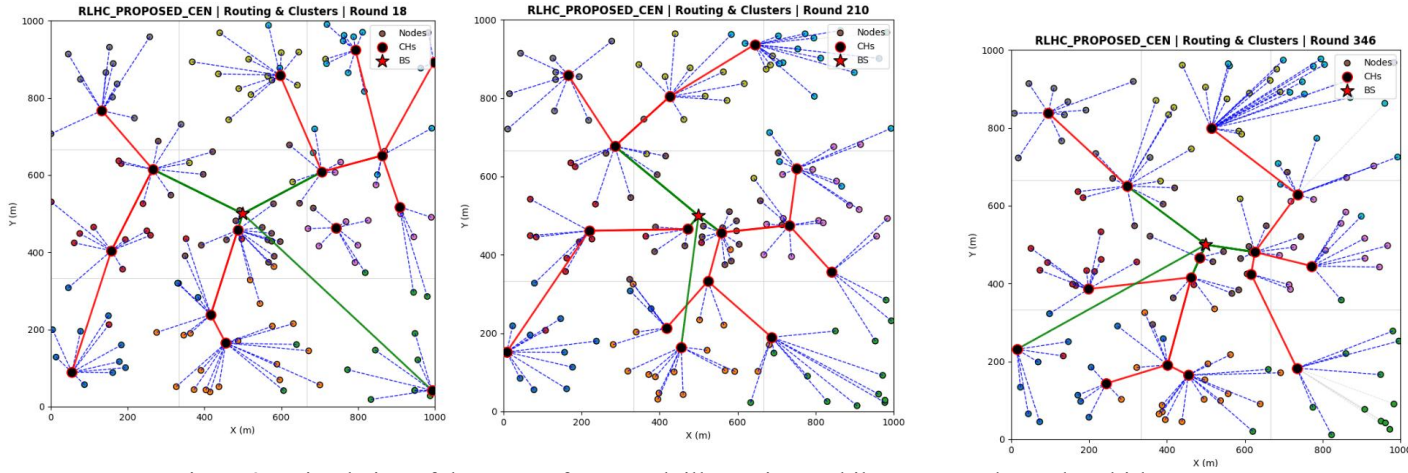
Figure 3.7 Simulation of the RLHC framework illustrating mobile sensor nodes and multi-hop communication
