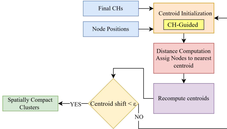
Figure 3.3.1 K-Means Algorithm
